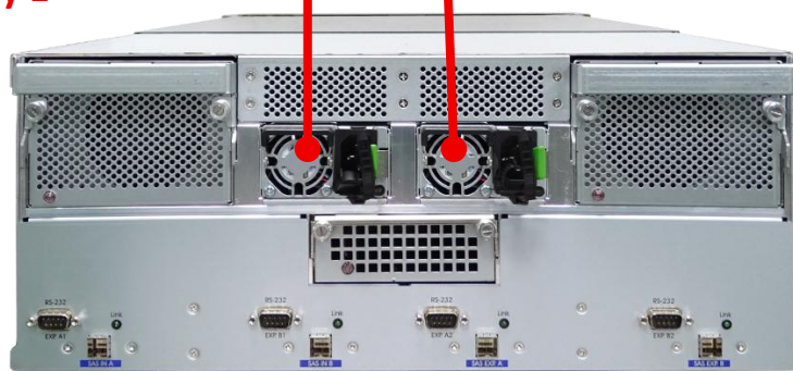
Power Supply 1 Power Supply 2
