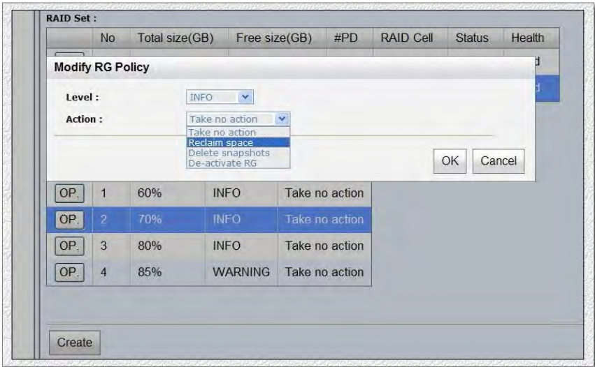
Figure 7: Space reclamation
